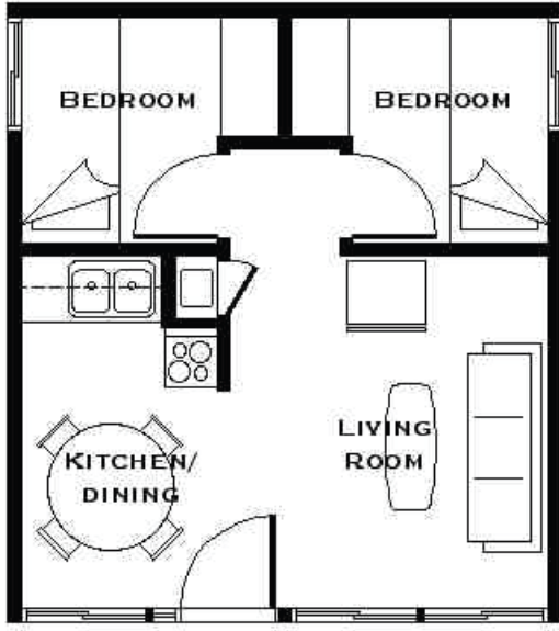
Reneker cabin layout
